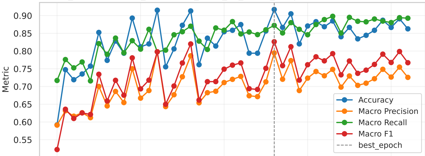
custom_cnn (Run: data_resampled_2025_12_11-22_35) | Accuracy/Precision/Recall/F1
