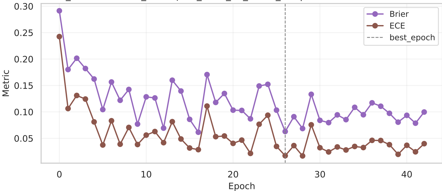
custom_cnn (Run: data_resampled_2025_12_11-22_35) | Calibration metrics (Brier/ECE)
