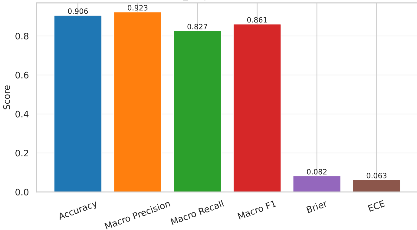
efficientnet_b1 | test (calibrated) metrics
