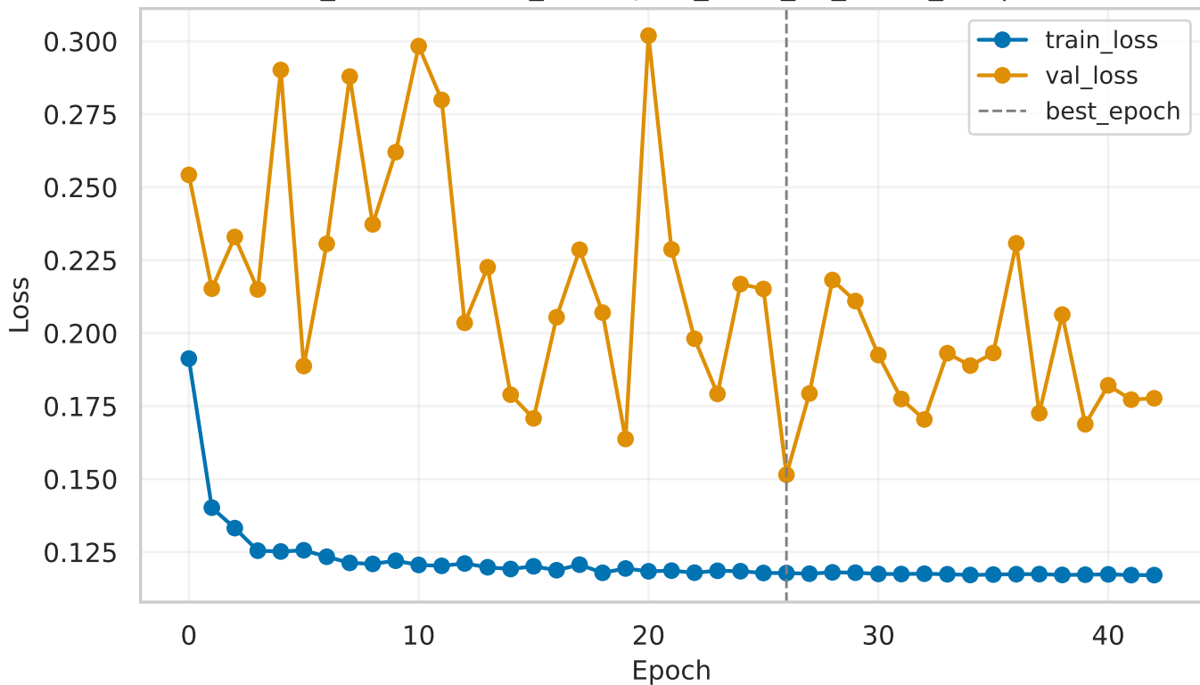
efficientnet_b1 (Run: data_resampled_2025_12_11-22_35) | Loss curves
