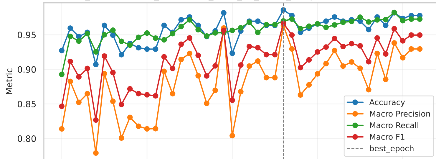
efficientnet_b1 (Run: data_resampled_2025_12_11-22_35) | Accuracy/Precision/Recall/F1
