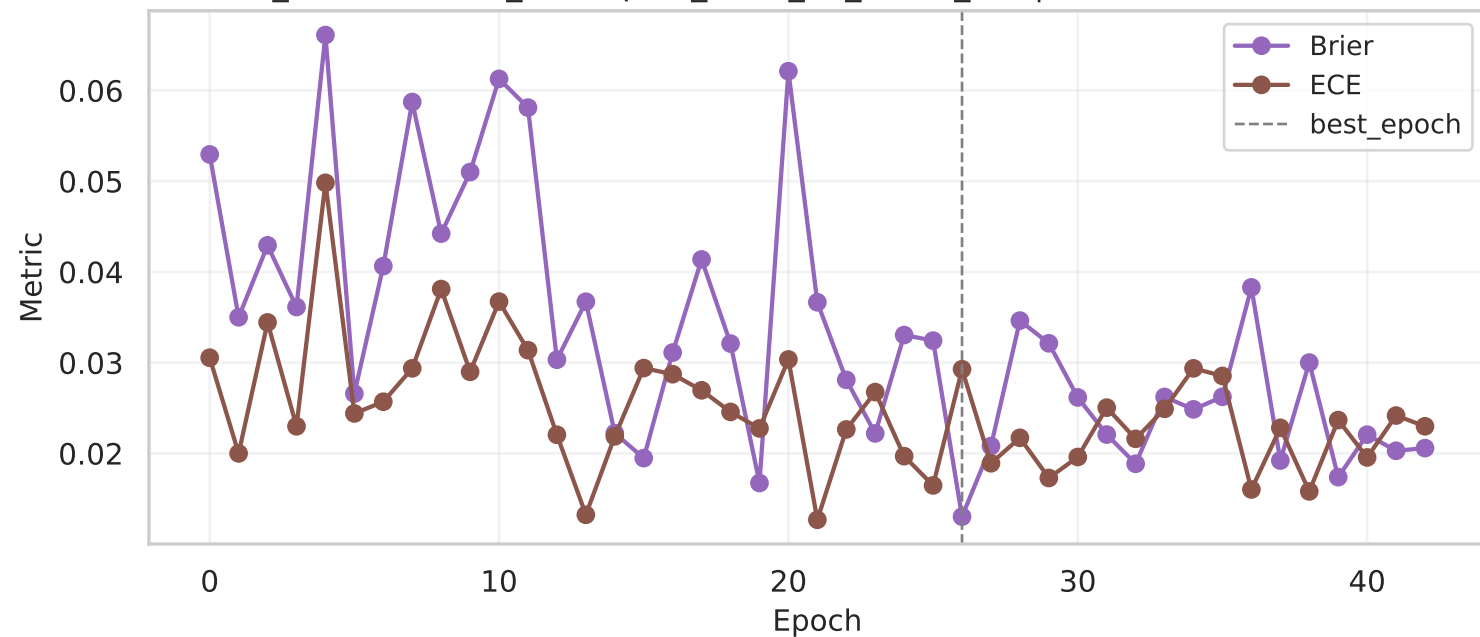
efficientnet_b1 (Run: data_resampled_2025_12_11-22_35) | Calibration metrics (Brier/ECE)
