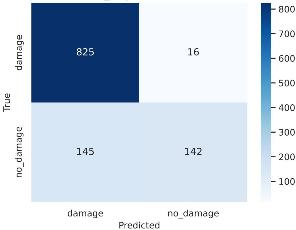
efficientnet_b2 | test Confusion (raw)
