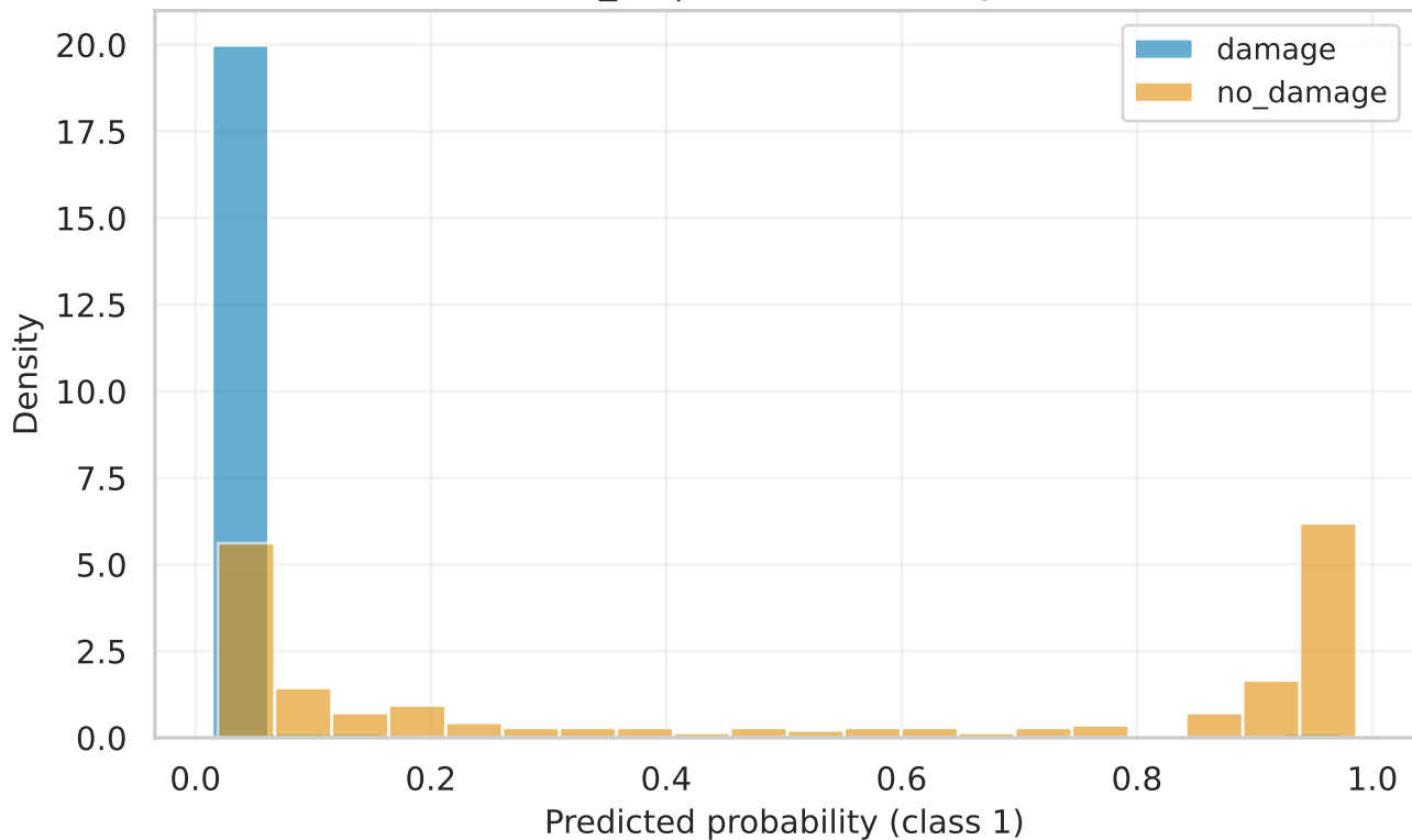
efficientnet_b2 | test Score Histogram (raw)
