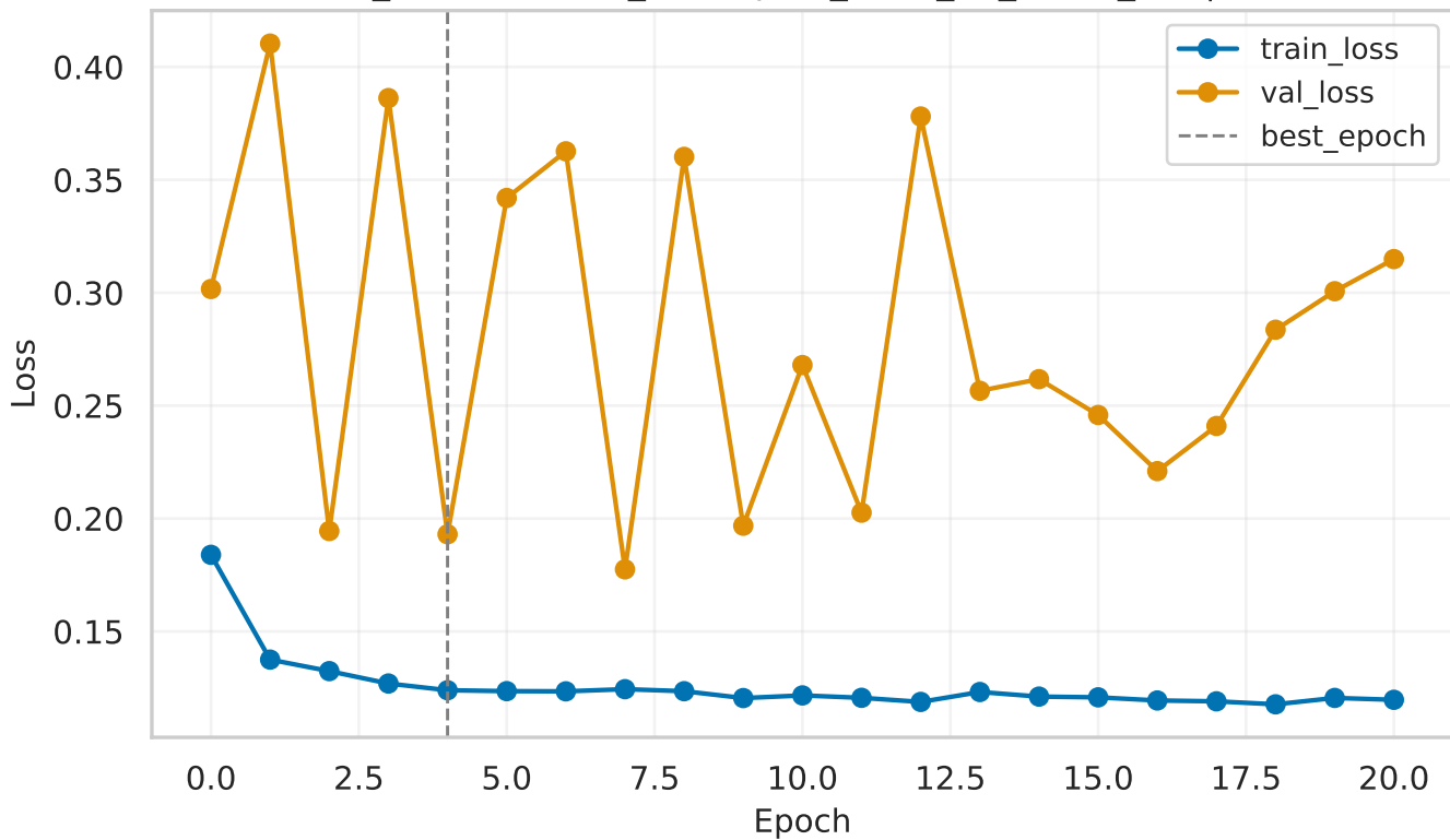
efficientnet_b2 (Run: data_resampled_2025_12_11-22_35) | Loss curves
