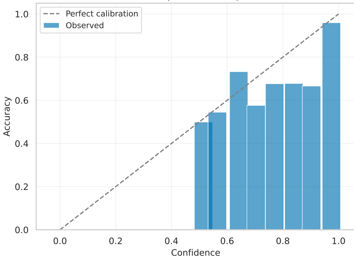
resnet18 | test Reliability (raw)
