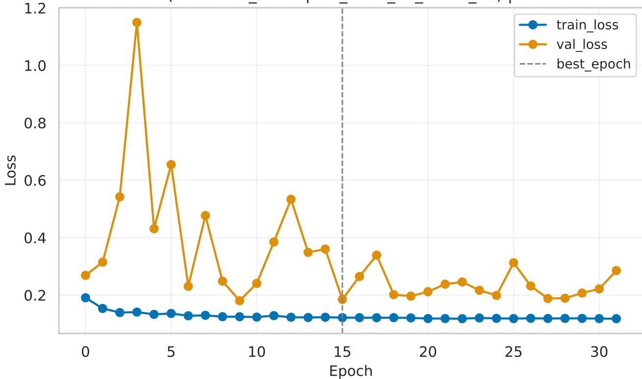
resnet18 (Run: data_resampled_2025_12_11-22_35) | Loss curves
