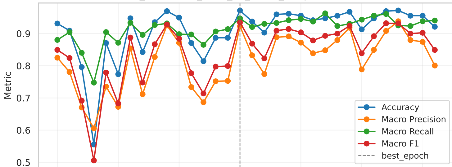
resnet18 (Run: data_resampled_2025_12_11-22_35) | Accuracy/Precision/Recall/F1
