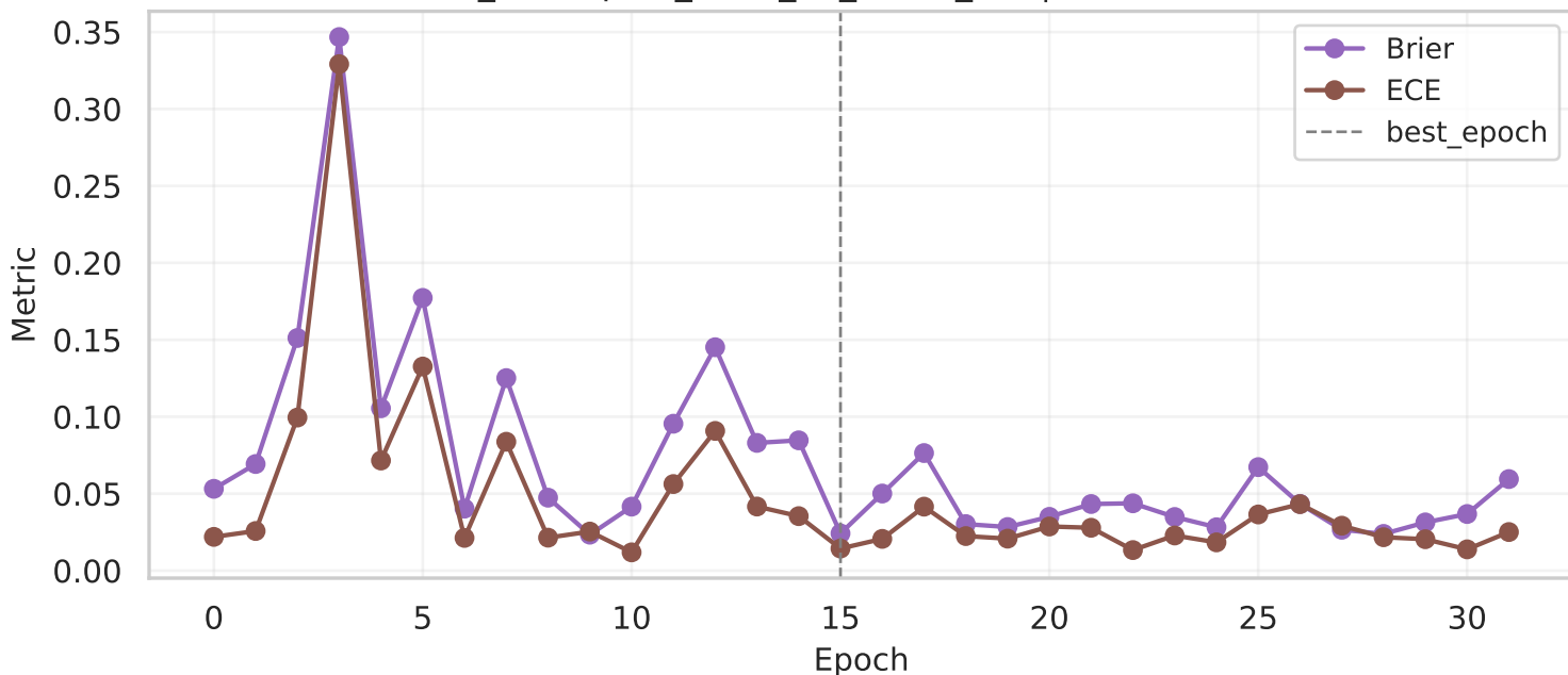
resnet18 (Run: data_resampled_2025_12_11-22_35) | Calibration metrics (Brier/ECE)
