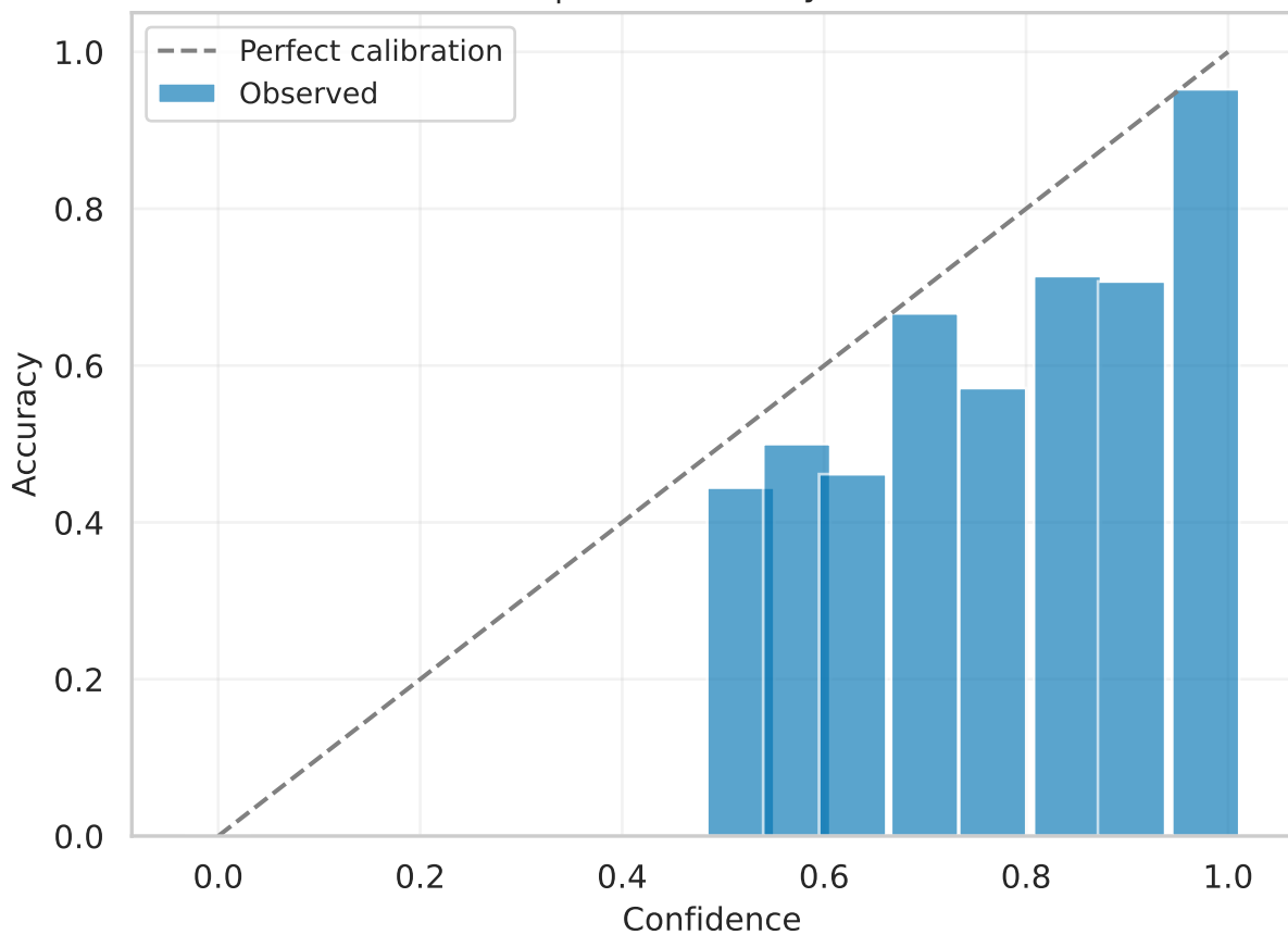
resnet34 | test Reliability (calibrated)
