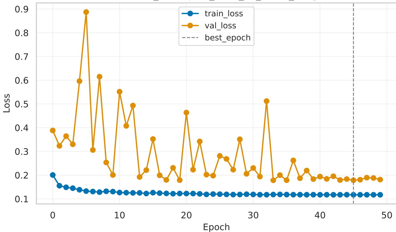
resnet34 (Run: data_resampled_2025_12_11-22_35) | Loss curves
