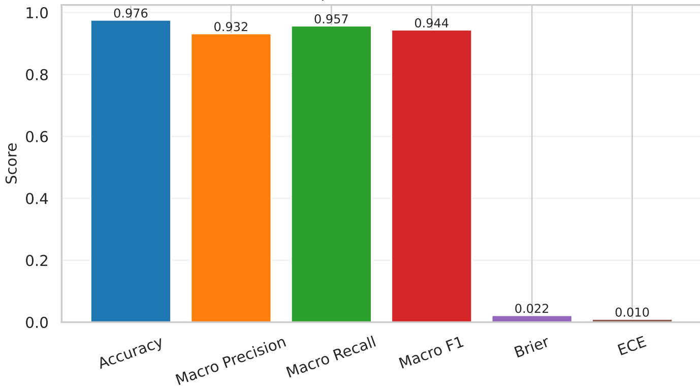
resnet50 | val (calibrated) metrics
