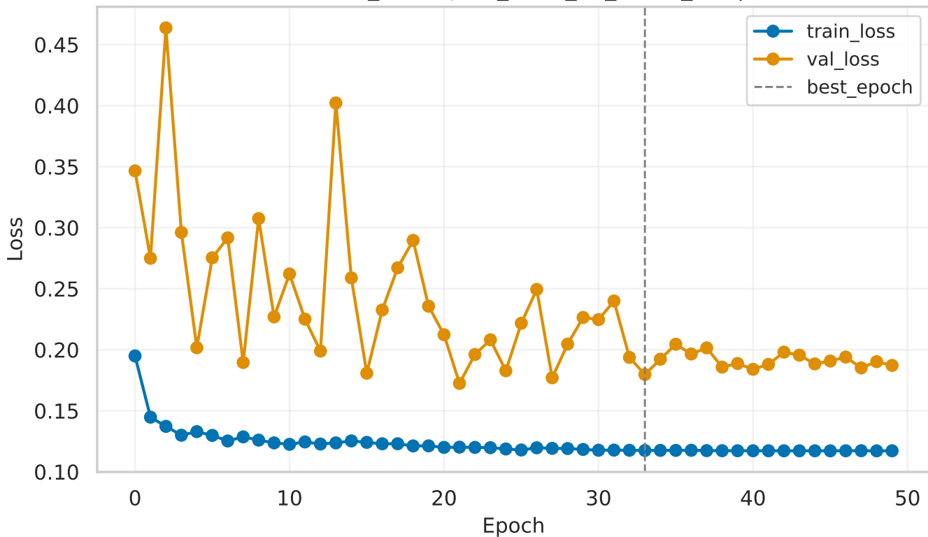
resnet50 (Run: data_resampled_2025_12_11-22_35) | Loss curves
