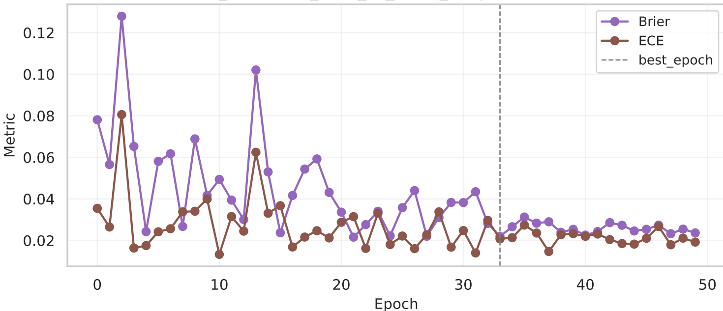
resnet50 (Run: data_resampled_2025_12_11-22_35) | Calibration metrics (Brier/ECE)
