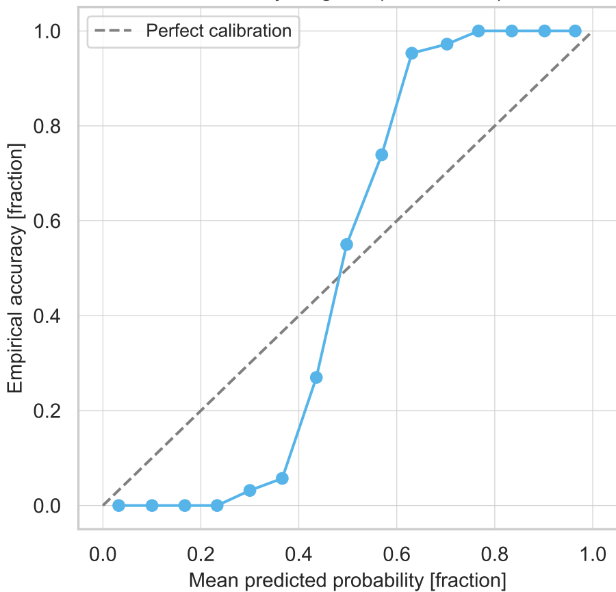
Reliability diagram (ECE=0.177)
