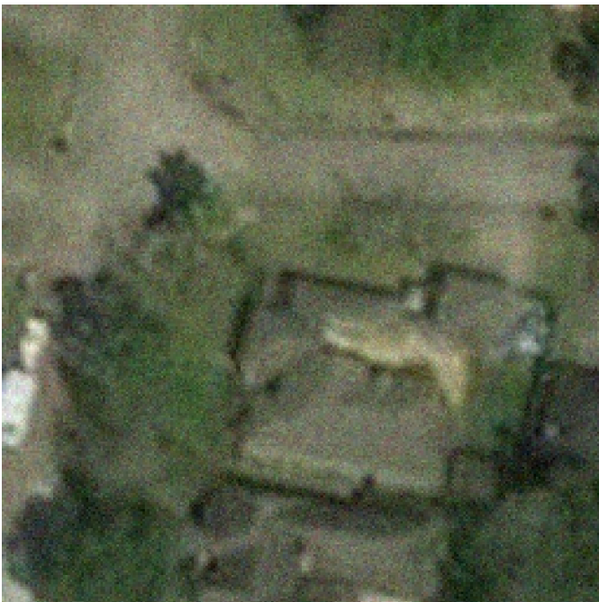
test/no_damage,-95.637139_29.840113.jpeg
