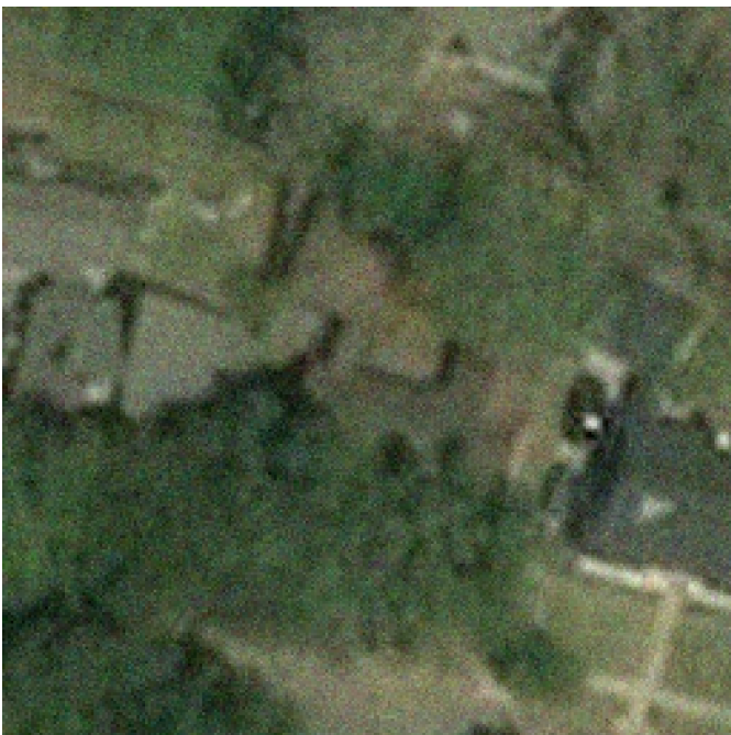
test/no_damage,-95.635708999999999_29.772269.jpeg
