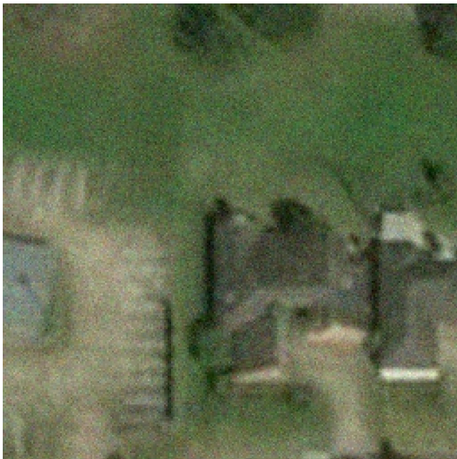
test/no_damage,-95.627952000000001_29.864295000000002.jpeg
