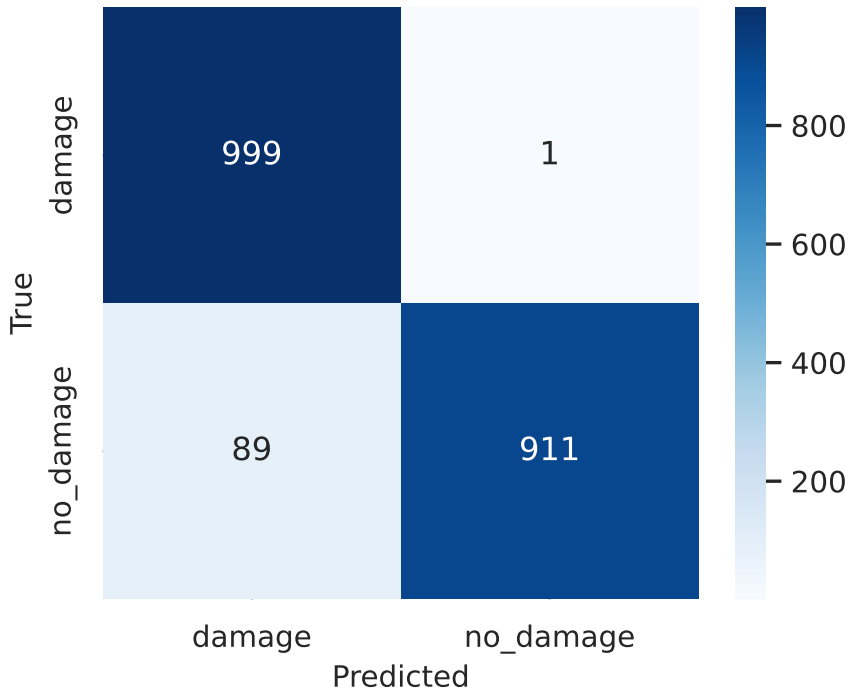
Val Confusion Matrix
