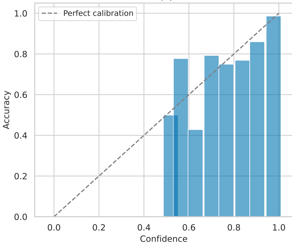
Test Reliability | ECE=0.021
