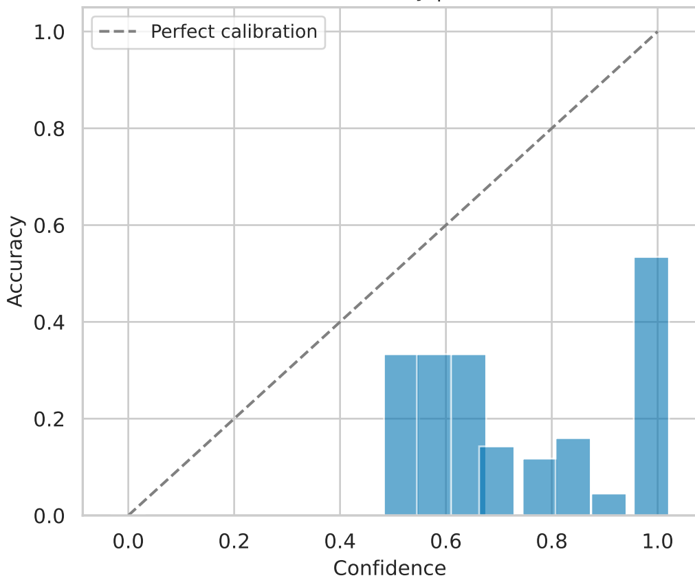
Validation Reliability | ECE=0.466
