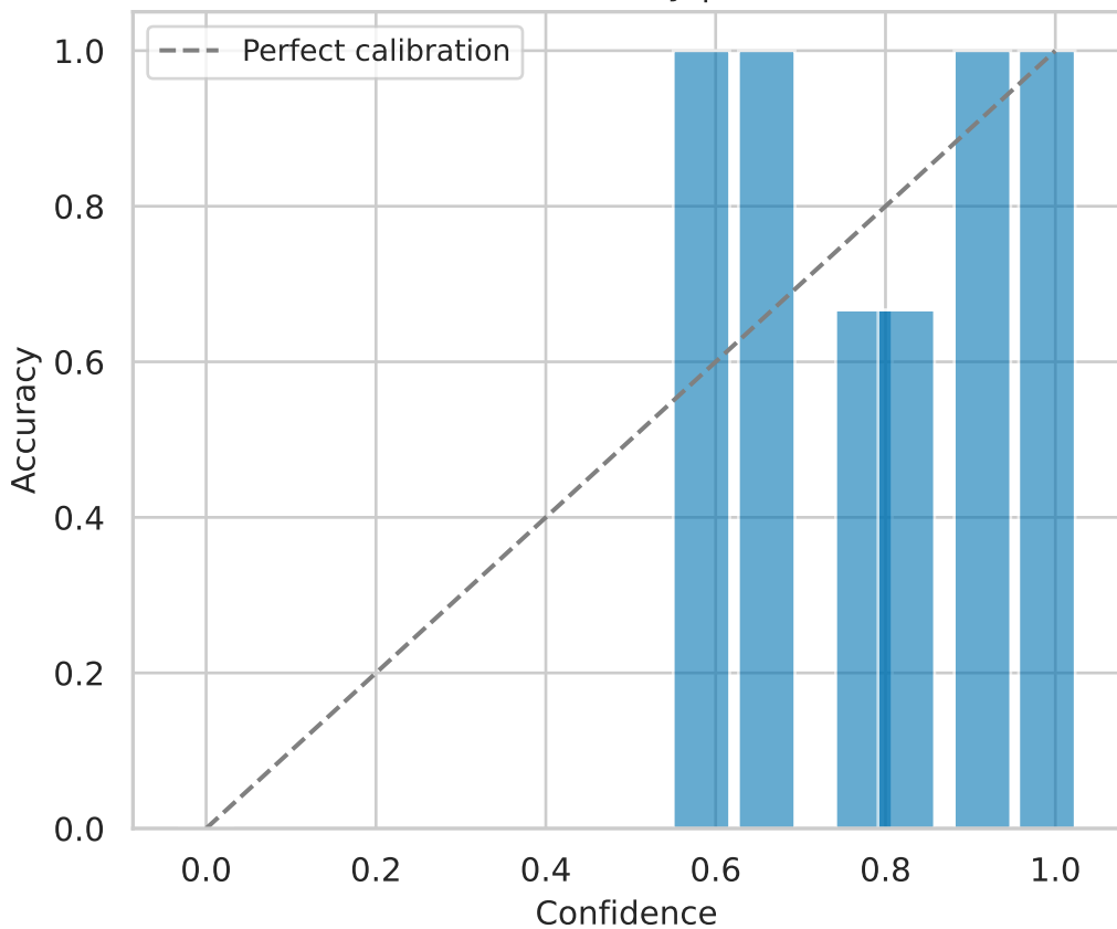
Validation Reliability | ECE=0.011
