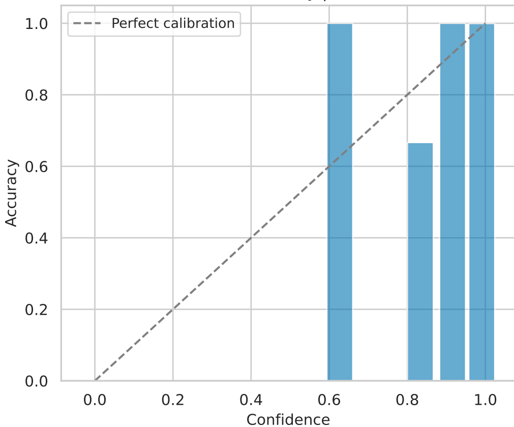
Validation Reliability | ECE=0.009
