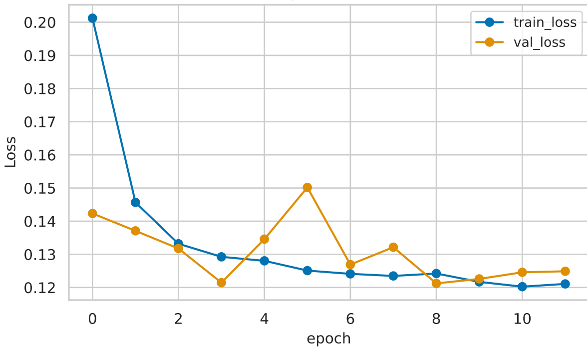
Training/Validation Loss
