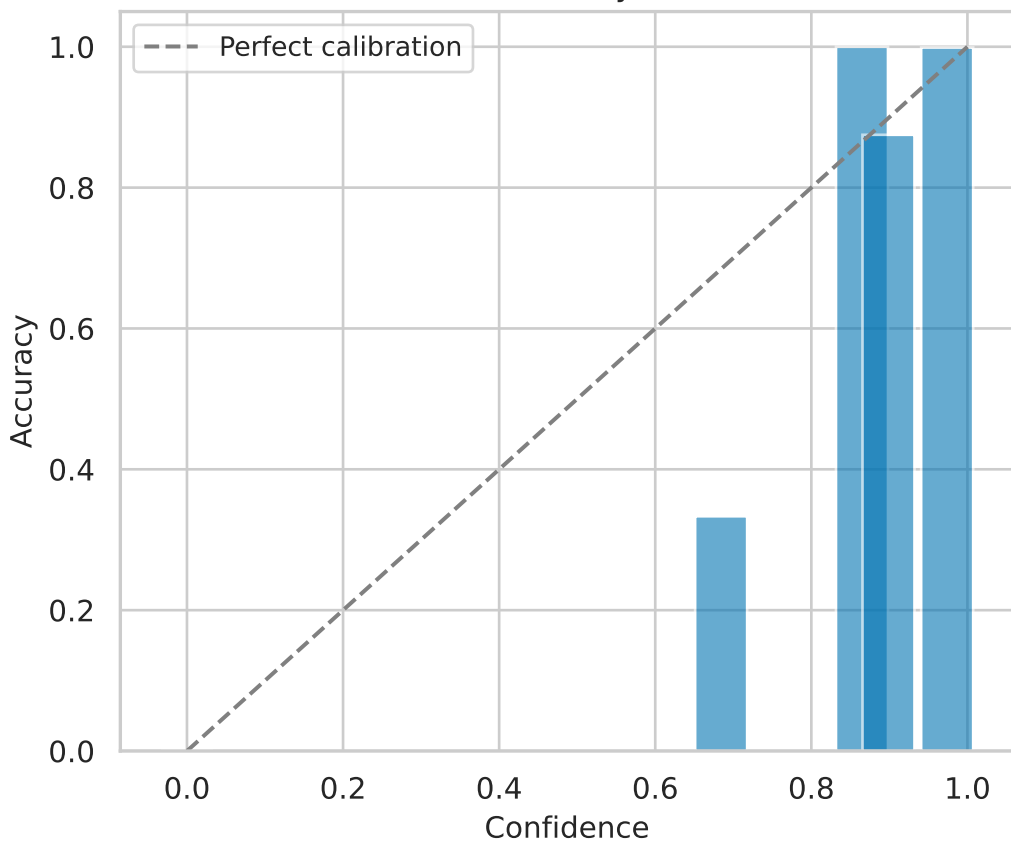
test Reliability (raw)
