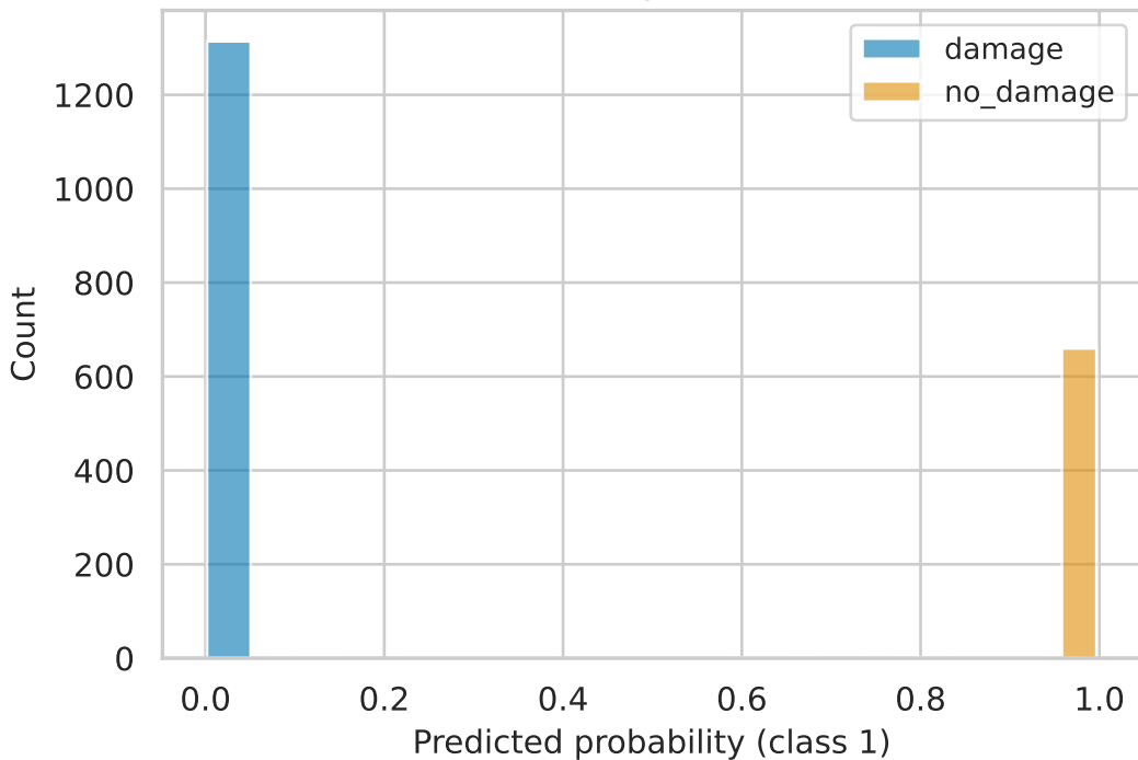
test Score Histogram (calibrated)
