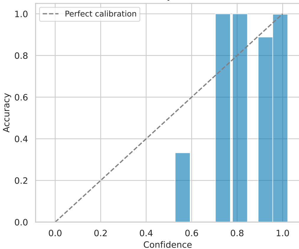
test Reliability (calibrated)
