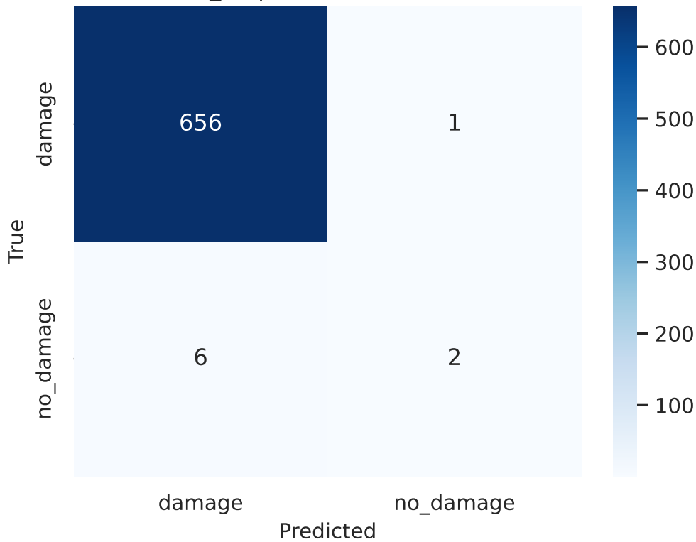
efficientnet_b1 | test Confusion (calibrated)
