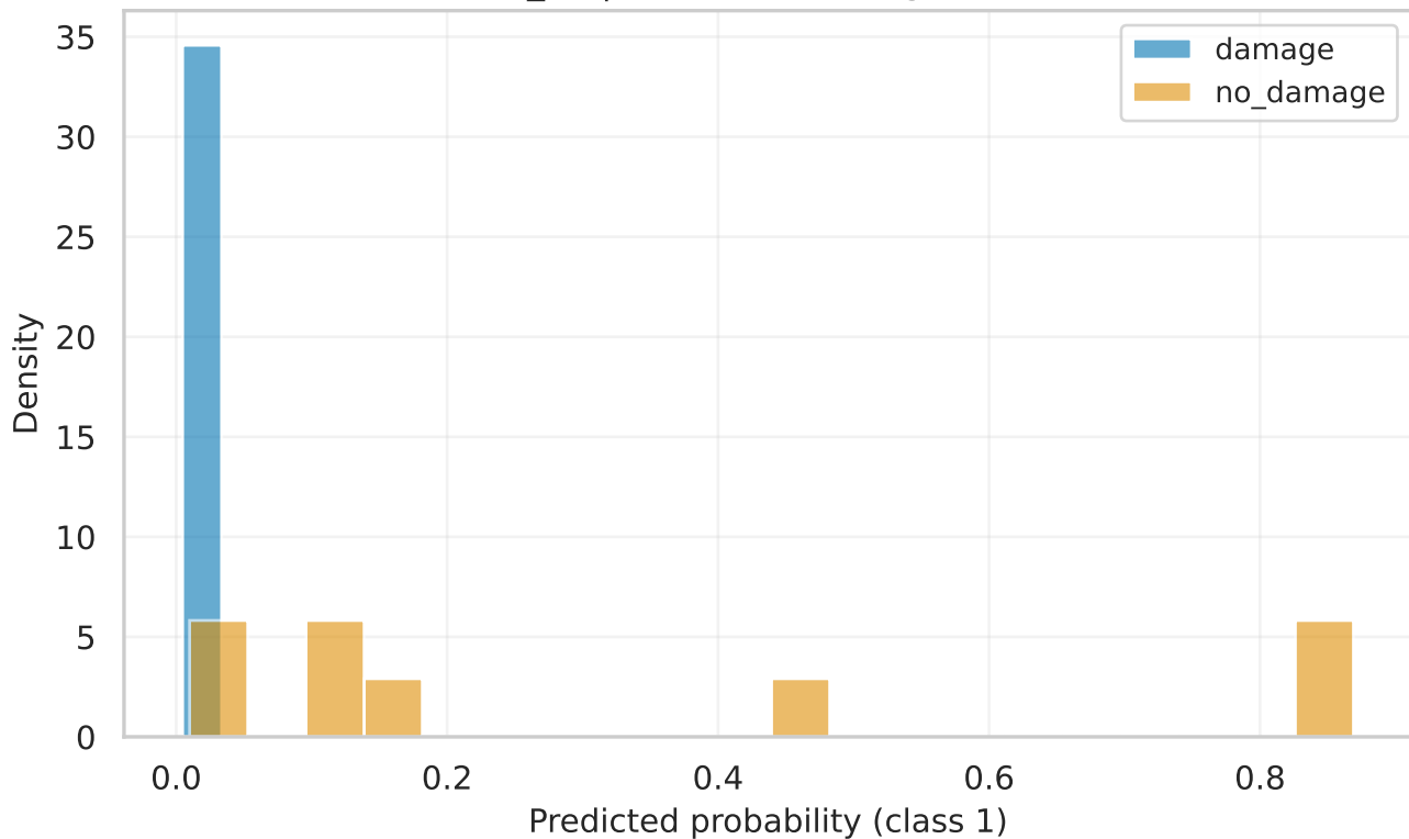
efficientnet_b1 | test Score Histogram (calibrated)
