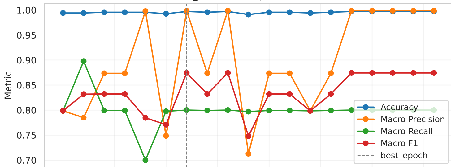
efficientnet_b1 | Accuracy/Precision/Recall/F1
