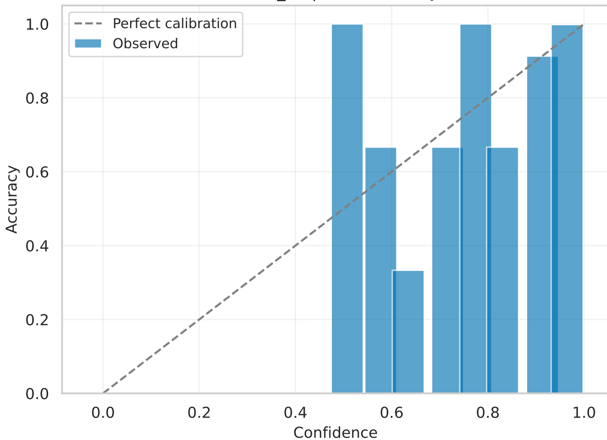
efficientnet_b2 | test Reliability (raw)
