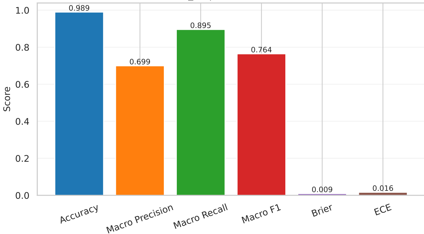
efficientnet_b2 | val (calibrated) metrics
