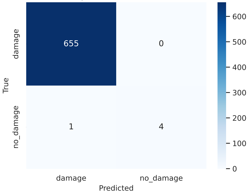
resnet18 | val Confusion (calibrated)
