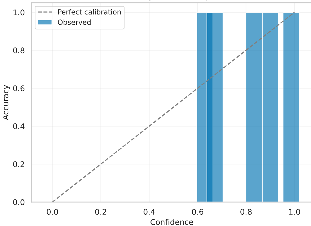
resnet18 | val Reliability (raw)
