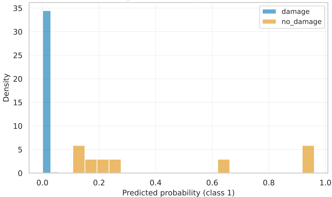
resnet18 | test Score Histogram (calibrated)
