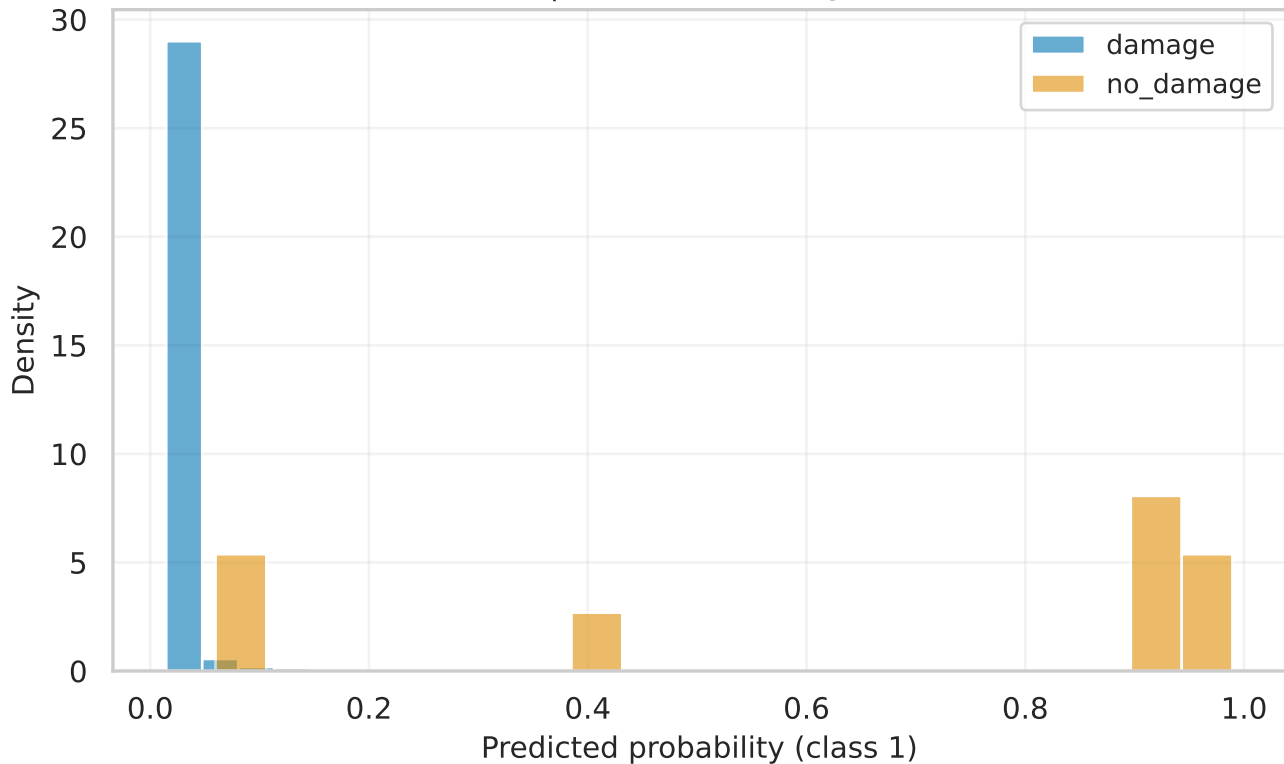
resnet34 | test Score Histogram (raw)
