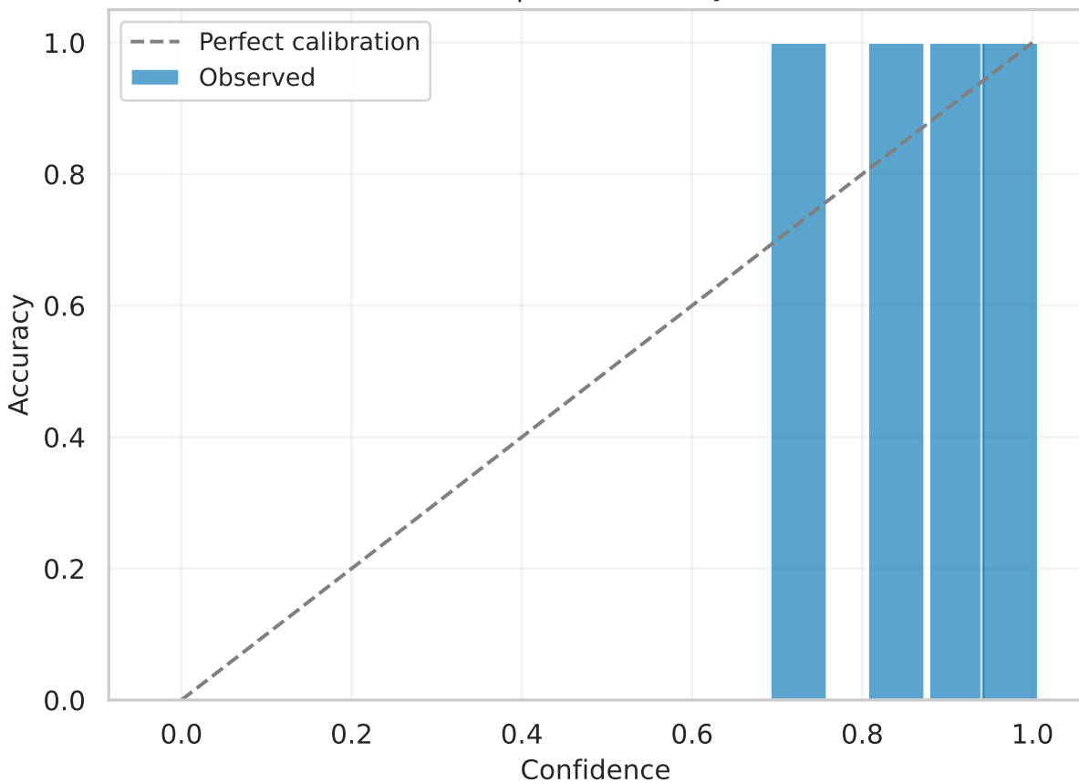
resnet34 | val Reliability (raw)
