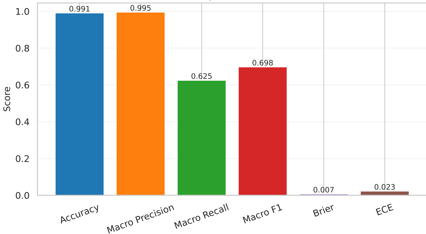
resnet50 | test (raw) metrics
