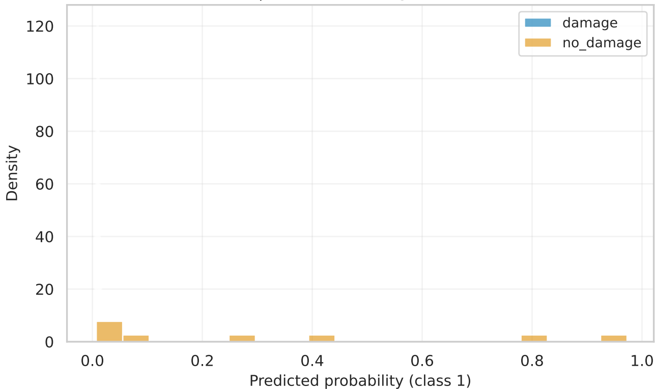
resnet50 | test Score Histogram (calibrated)
