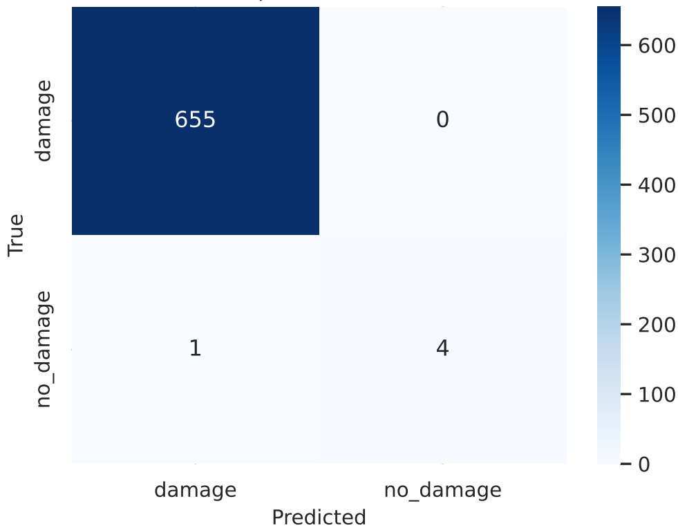
resnet50 | val Confusion (raw)
