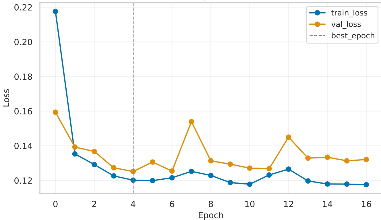
resnet50 | Loss curves
