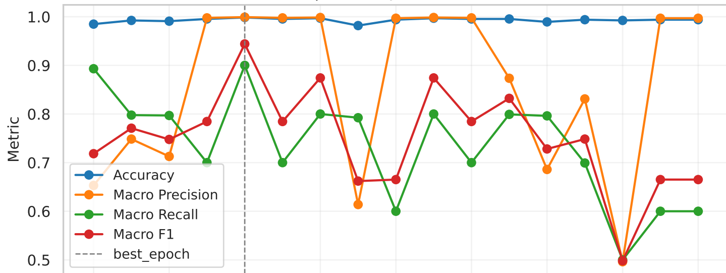
resnet50 | Accuracy/Precision/Recall/F1
