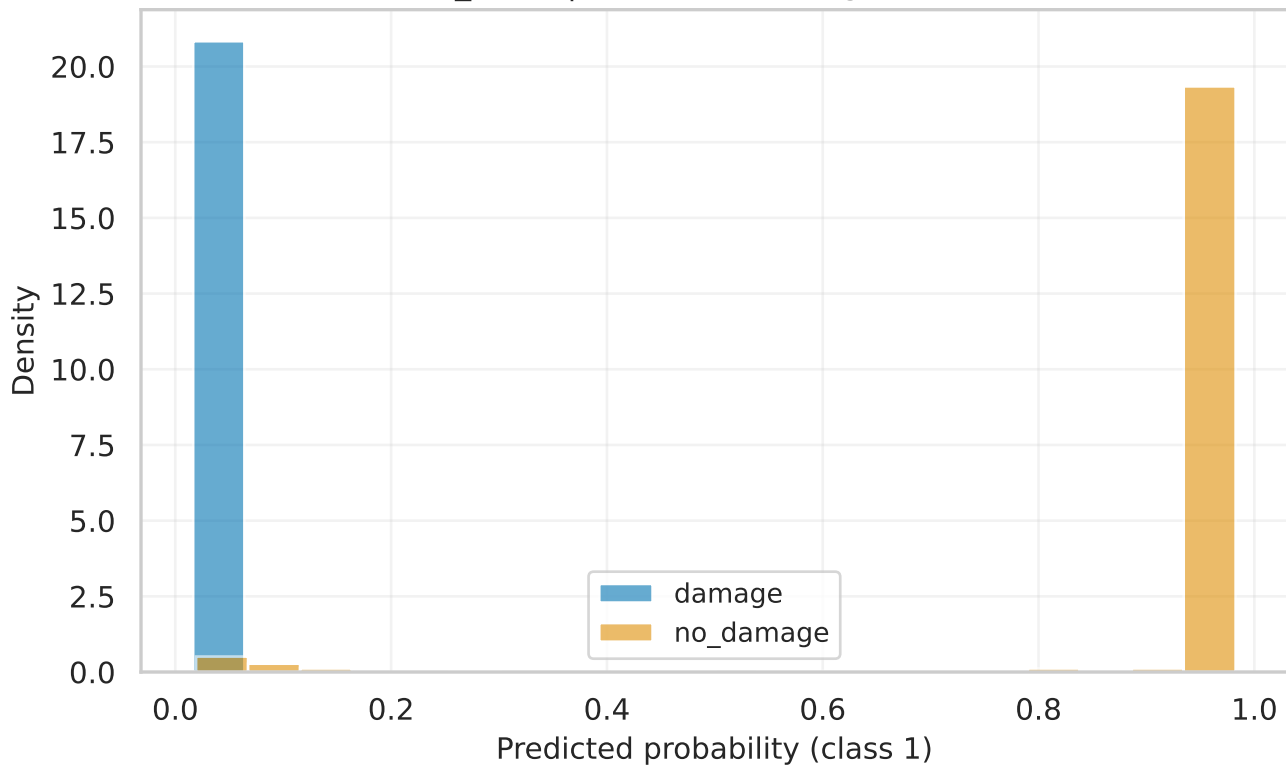
convnext_small | test Score Histogram (calibrated)
