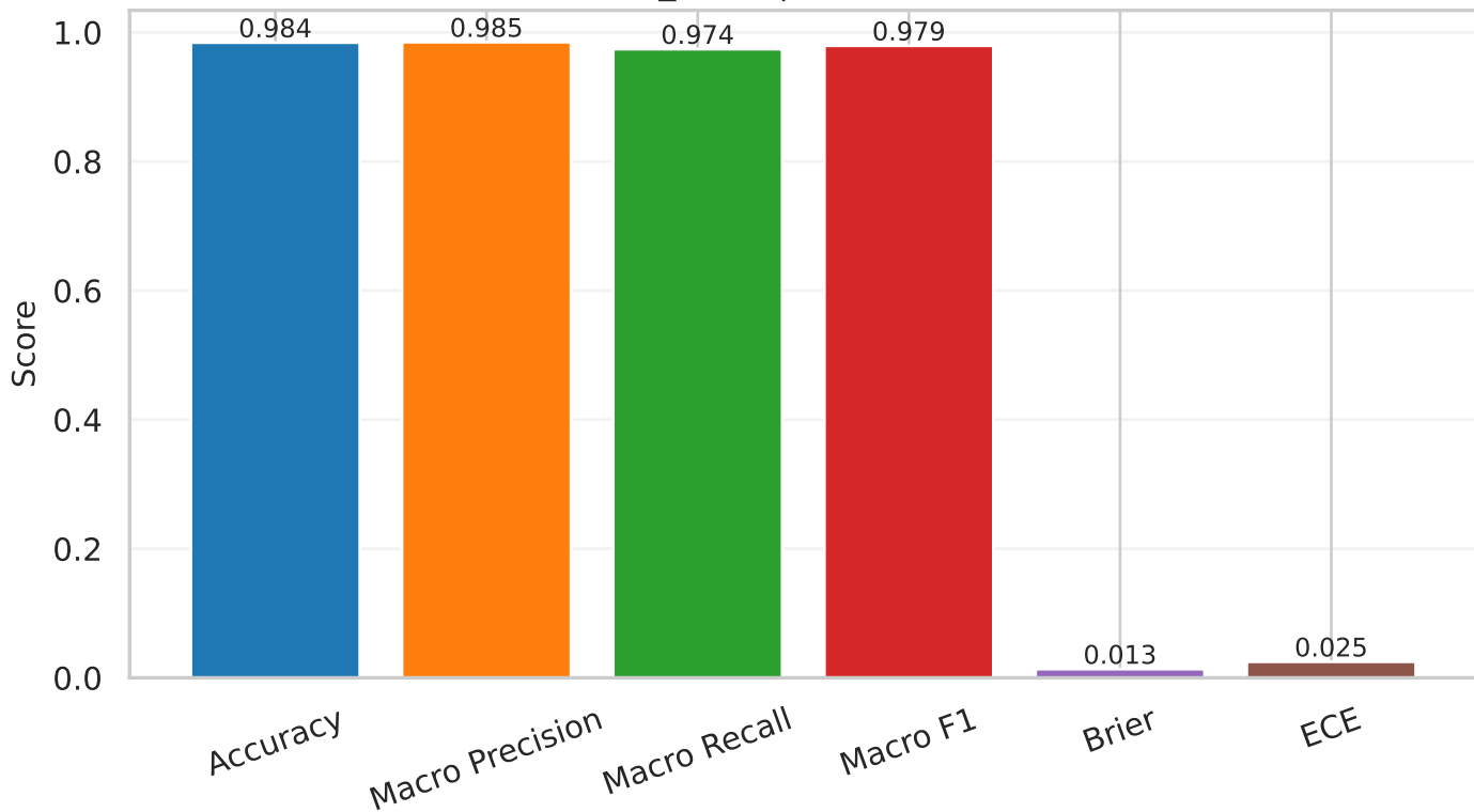
convnext_small | test (raw) metrics
