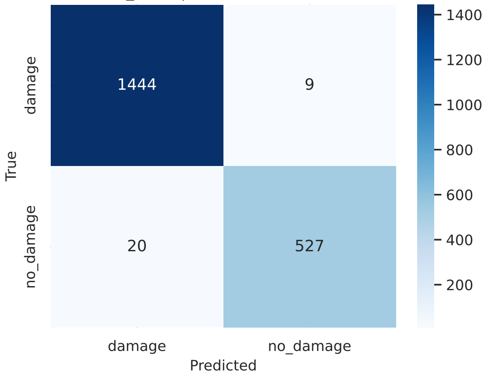
convnext_small | val Confusion (calibrated)
