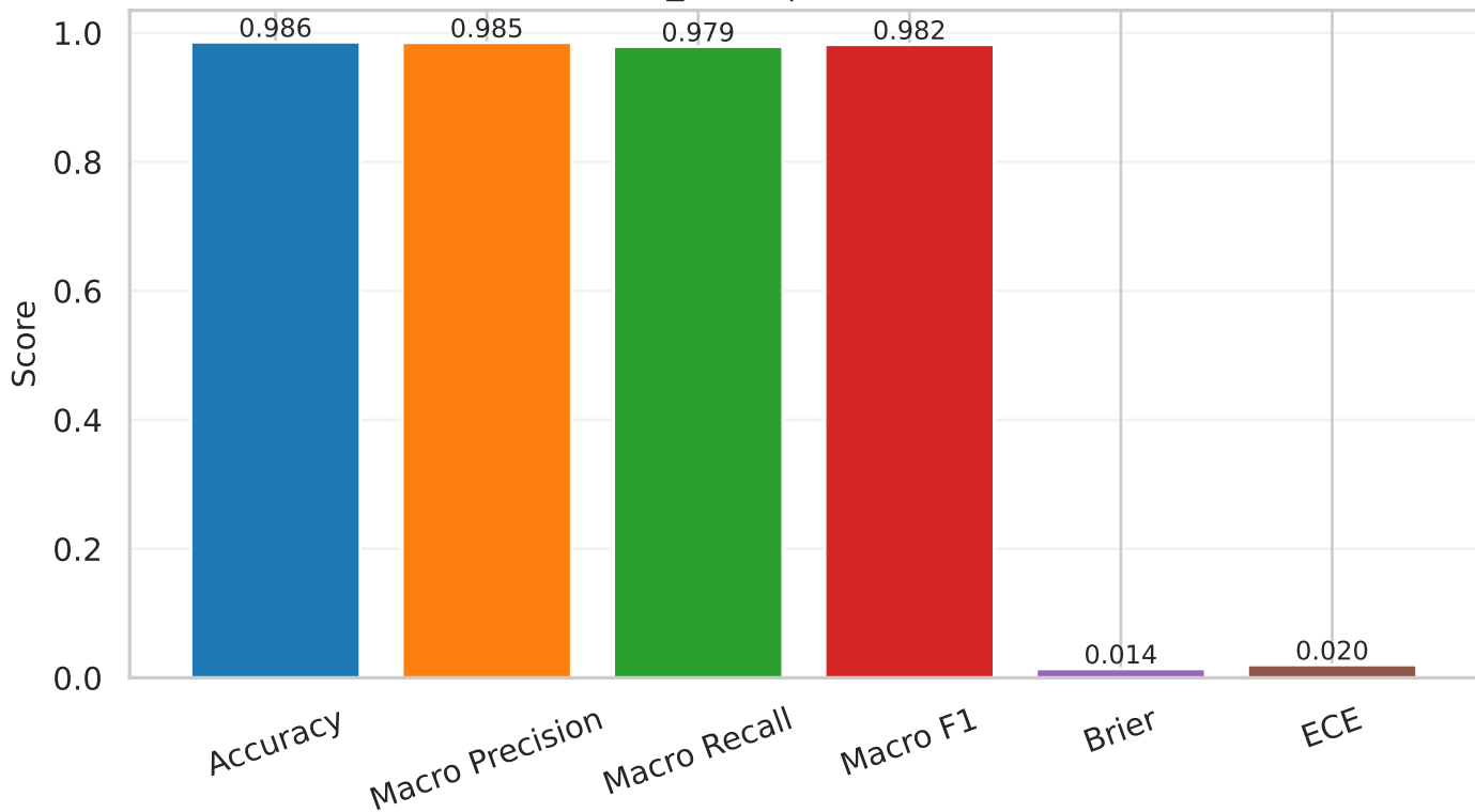
convnext_small | val (raw) metrics
