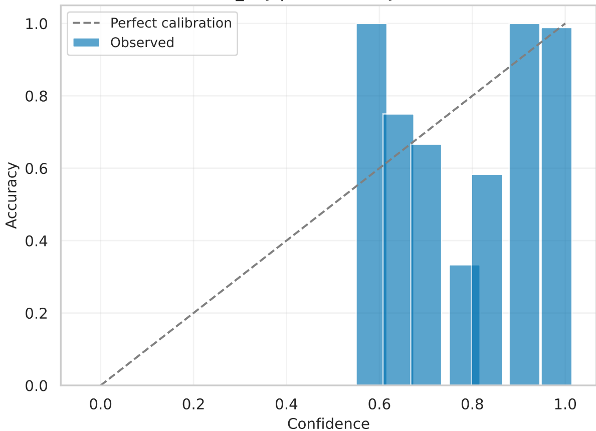
convnext_tiny | val Reliability (calibrated)
