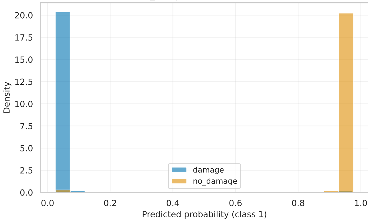
convnext_tiny | val Score Histogram (raw)
