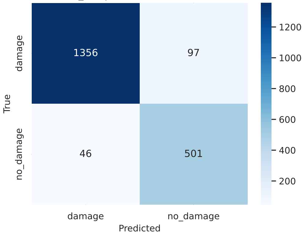
custom_cnn | val Confusion (calibrated)
