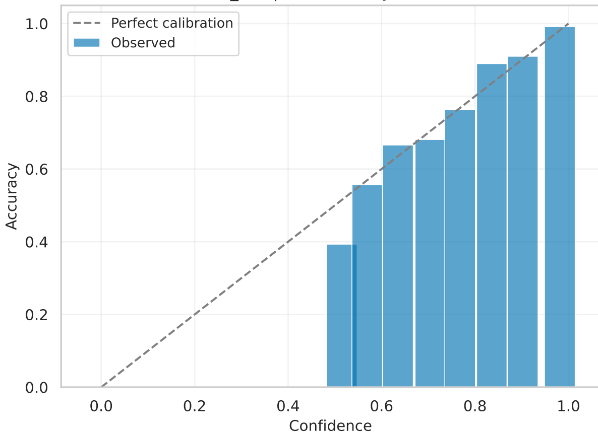
custom_cnn | val Reliability (calibrated)
