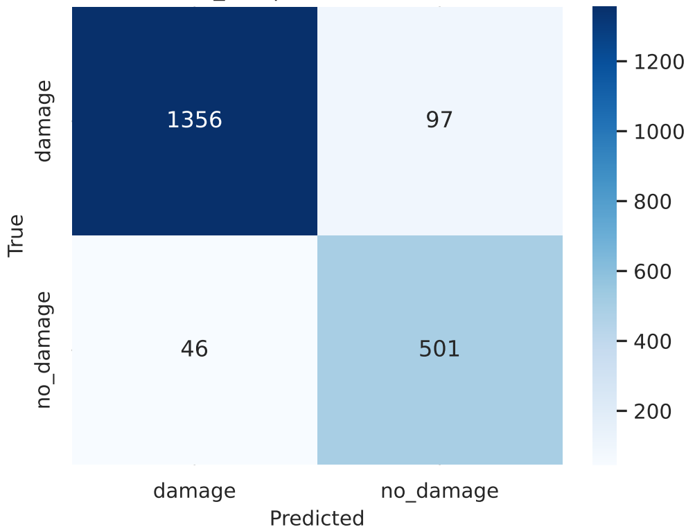
custom_cnn | val Confusion (raw)
